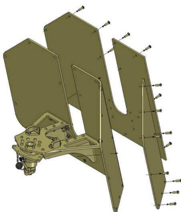
Front Shield Kit (STANAG Level 1,2,3)
